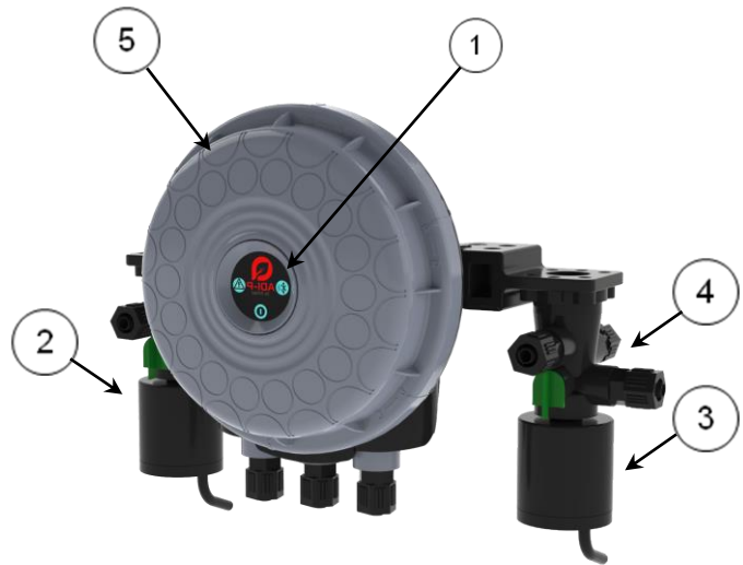
Dual solenoid controller
