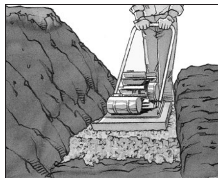
Diagram 2 – Leveling Pad
