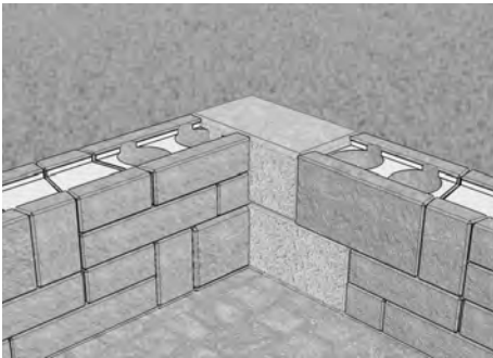
16" Freestanding Wall Pattern
