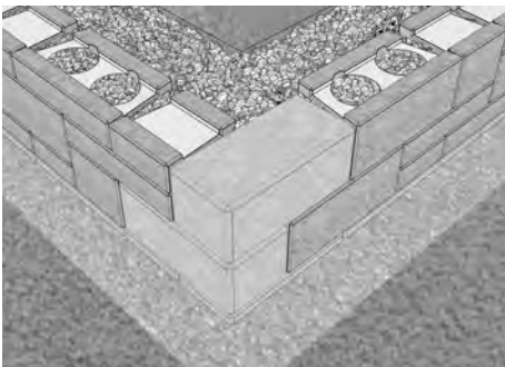
16" Retaining Wall Pattern
