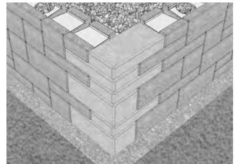
32" Retaining Wall Pattern
