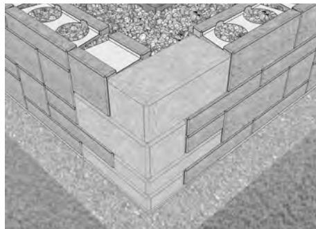
24" Retaining Wall Pattern
