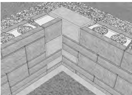
32" Retaining Wall Pattern
